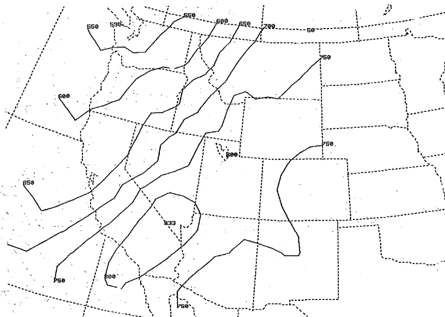
Figure 2 314K isentropic pressure field for 12Z, August 13, 1984.
