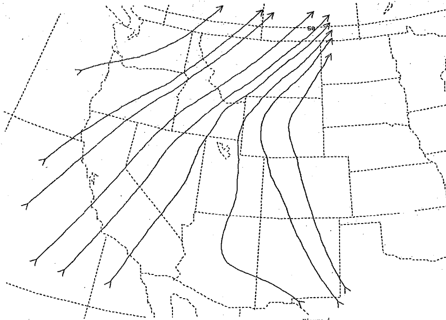
Figure 4 314K Streamlines for 12Z, August 13, 1984.
