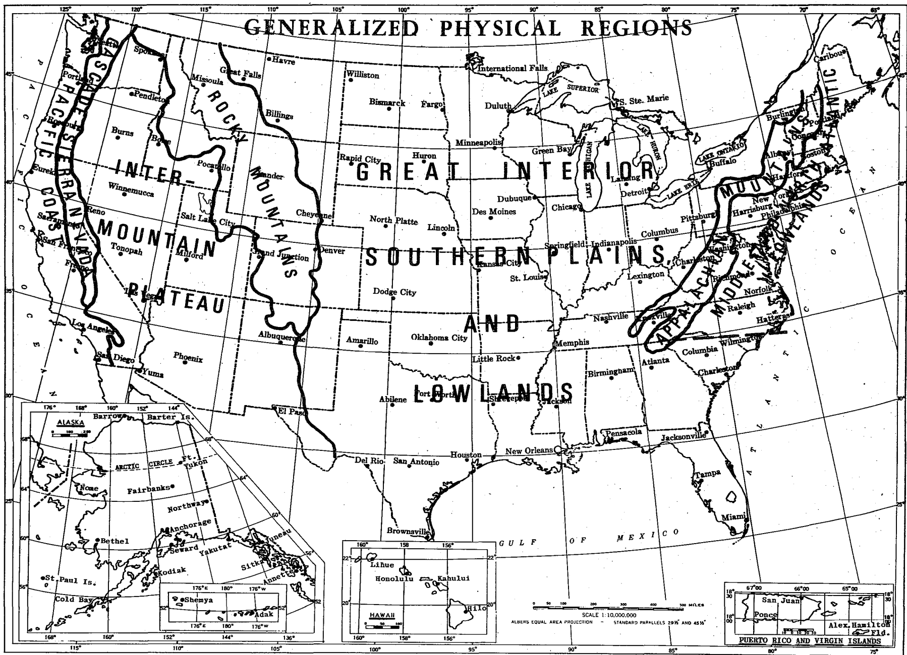
Figure 1. Geographic Regions of the United States (Baldwin, 1973)
