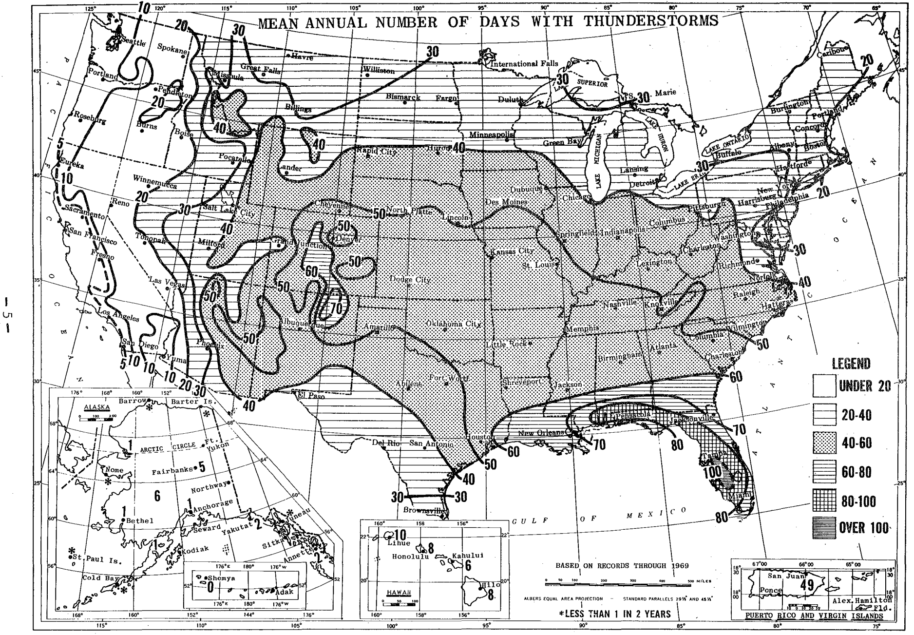
Figure 3. Mean Annual Number of Thunderstorm Days (Baldwin, 1973)
