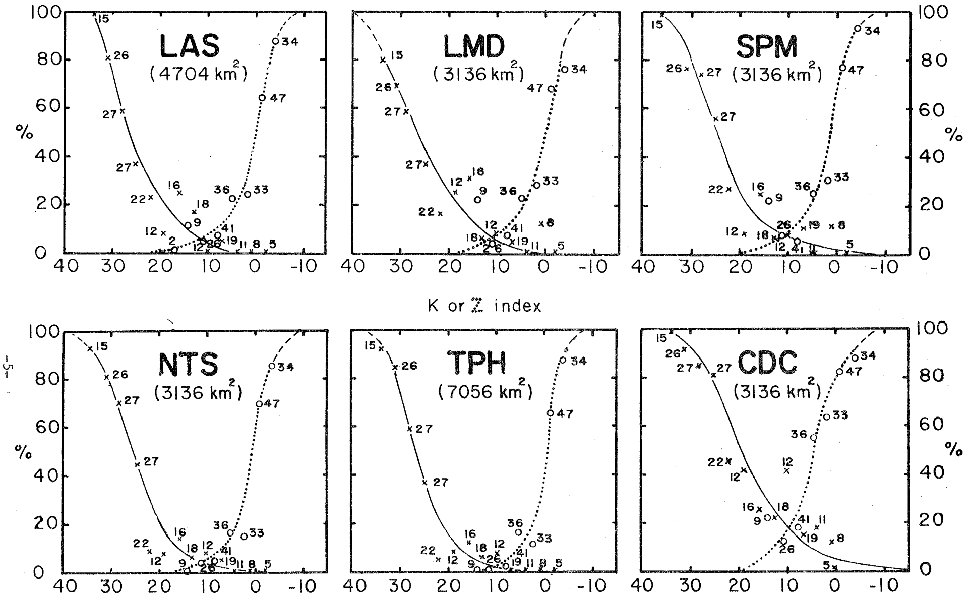
Figure 3. Relative frequency of occurrence of an echo-day for specified areas between local midnight and local midnight as a function of K and Z index values calculated from the Yucca Flat 1200Z sounding. The K curve is represented by the solid line, the Z curve by the dotted line. Values plotted next to the x's are the number of days in each K category and the numbers next to the o's are the number of days in each Z category.
