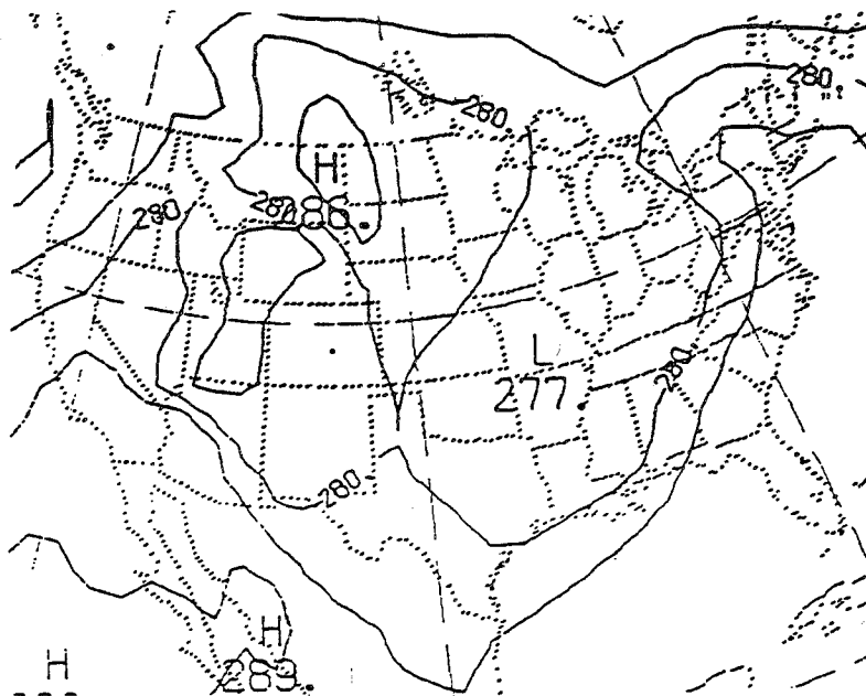
Fig. 5 48 Hour forecast 850 mb temperatures from the operational NCM initialized on 25 October 1986.
