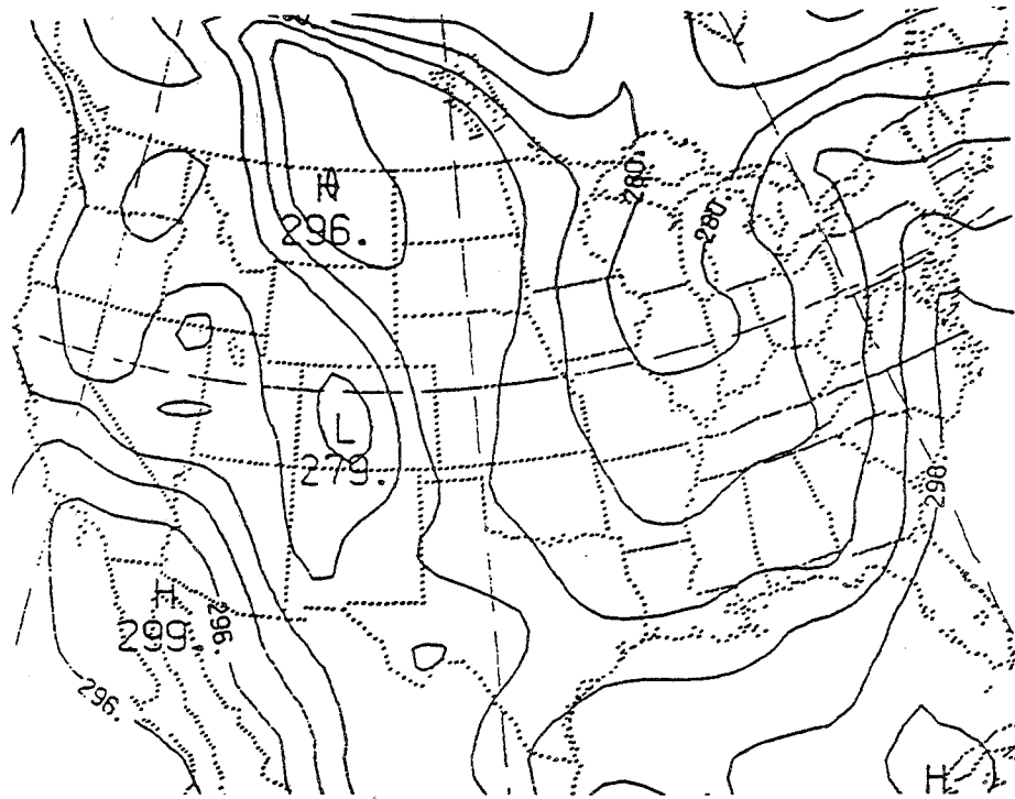
Fig. 4 48 Hour forecast first sigma layer temperatures from the NCM without the physics package initialized on 25 October 1986.
