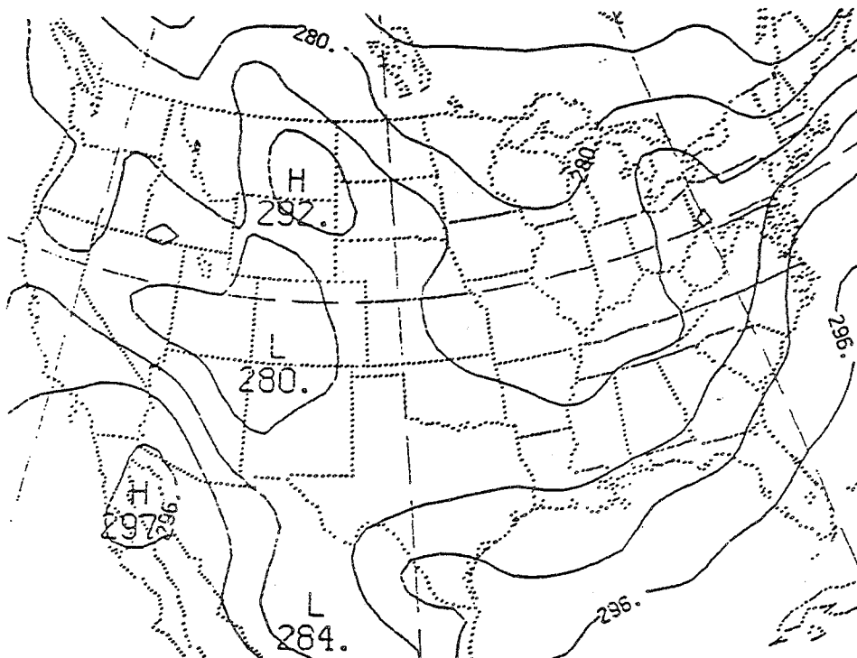
Fig. 8 00 Hour forecast first sigma layer temperatures initialized on 27 October 1986.
