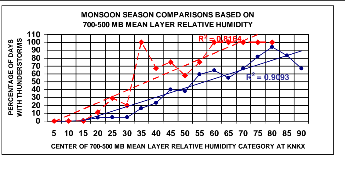
Fig. 6. Figure shows the percentage of days with thunderstorms in the WFO San Diego County Warning and Forecast Area (CWFA) in comparison to the maximum 700-500 mb mean layer relative humidity of the day at the Miramar (KNKX) sounding. The blue curve with the circles was constructed using the available data for June-September of 2003-2005 (Thunderstorm data was unavailable before summer 2003). A total of 301 of a possible 305 days were available. The blue line is the trend line for the curve, showing a very high correlation of 0.91. The dashed red curve with the diamonds and dashed trend line are for 1 June – 31 July 2006 (61 of a possible 61 days of data available). One feature that stands out is the curves for the 2006 event have a much higher incidence of thunderstorms compared to the 2003-2005 curves for the same relative humidity values. This may indicate more favorable conditions during the 2006 period due to factors such as wind direction from the continent and the increased number of easterly waves and upper low episodes caught up in the “fast” easterly flow beneath the monsoonal high. On some days thunderstorms beginning over the mainly higher terrain to the east simply “advected” into the forecast area. The high number of dynamically driven events may also help to explain the reduction in the correlation coefficient in 2006. For the purposes of this study the lower bound for an event to be labeled “monsoon” is 30 percent 700-500 mb relative humidity and any wind in the layer with a direction from 0 to 225 degrees. Notice that the 700-500 mb mean relative humidity and the percentage of days with thunderstorms is very similar based on the blue trend line for the 2003-2005 warm seasons. For this development data, the probability of a thunderstorm in the forecast area is slightly lower than the 700-500 mb layer mean relative humidity. (Simply reducing the 700-500 mb mean layer relative humidity by 7 is a good approximate of the probability of a thunderstorm as an initial estimate). The red curves are probably more applicable to a “dynamic” pattern with south (or possibly east) flow, and the blue curves are probably more applicable to a pattern with weak dynamics and south to east flow. For the “dynamic” cases, multiplying the mean 700-500 mb relative humidity by 1.5 is a good approximation of the probability of a thunderstorm. Typically, the most likely location of the first thunderstorms of the day (and sometimes the only area with thunderstorms) is the San Bernardino County Mountains, followed by either the San Diego County Mountains or the Apple and Lucerne Valleys. Only 3 years of data has been used for the blue curves, but they can still be used as a “reasonable estimate” of the character of the monsoon.
