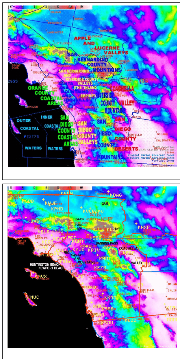
Fig. 1. Terrain maps of the WFO SGX County Warning and Forecast Area (CWFA). Color coding is in thousands of feet MSL.
