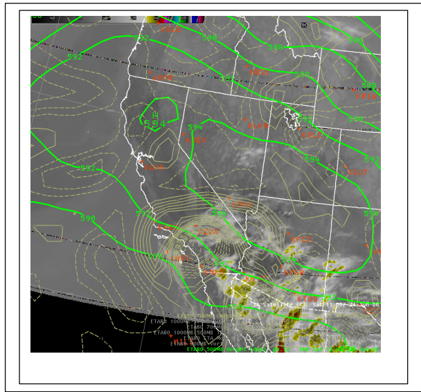
Fig. 7. The upper left panel is the 06 hour 500 mb forecast heights in decameters (green, solid) and the 700 mb vertical velocity in microbars per second (brown, dashed, and shaded) valid at 0600 UTC 24 June 2006. The upper right figure is the 00 hour 500 mb heights in decameters (green, solid) and the 700 mb vertical velocity in microbars per second (brown, dashed, and shaded) valid at 1200 UTC 24 June 2006. The lower left figure is the 0531 UTC infrared satellite imagery overlaid with the 06 hour 500 mb forecast heights in decameters (green, solid) and 700 mb vertical velocity in microbars per second (brown, solid and dashed) valid at 0600 UTC 24 June 2006. The lower right is the 1100 UTC 24 June 2006 infrared satellite imagery overlaid by the 00 hour 500 mb heights in decameters (green, solid) and the 700 mb vertical velocity in microbars per second (brown, dashed) valid at 1200 UTC 24 June 2006. The peaks in the downward vertical velocity (DVV) over the coastal waters and at the immediate coast during the two time periods were -2.6 and -4.4 respectively.
