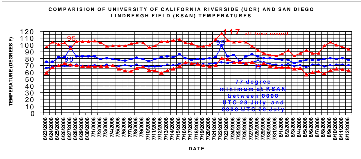
Fig. 3. The figure shows the high and low temperatures for the University of California Riverside (red with triangles) and San Diego Lindbergh Field (blue with circles). The temperatures are for the 24 hour period ending at 4 pm local standard time of the day in question. The peak San Diego temperatures of 96 and 99 degrees can be easily seen. The inversion top and 850 mb temperatures were 34.6 and 30.6 at 0000 UTC 23 July 2006. The overnight low temperature for the 24 hour period ending at 0000 UTC on 29 July 2006 was 77 degrees F. This 77 degree overnight low temperature occurred close to the sea surface temperature maximum of 80 degrees F at Huntington Beach at 1700 UTC 29 July 2006. (The all time record for a calendar day at KSAN is 78 degrees F). The strong modulating affect of the clouds on 27 June 2006 is reflected in the high temperature at San Diego (at the coast) exceeding the high temperature at Riverside (in the inland valley area), a rare event during the summer. Also, the extremely high 850 mb dewpoint peak was 15.6 degrees C at 0000 UTC 28, which helps to keep minimum temperatures up.
