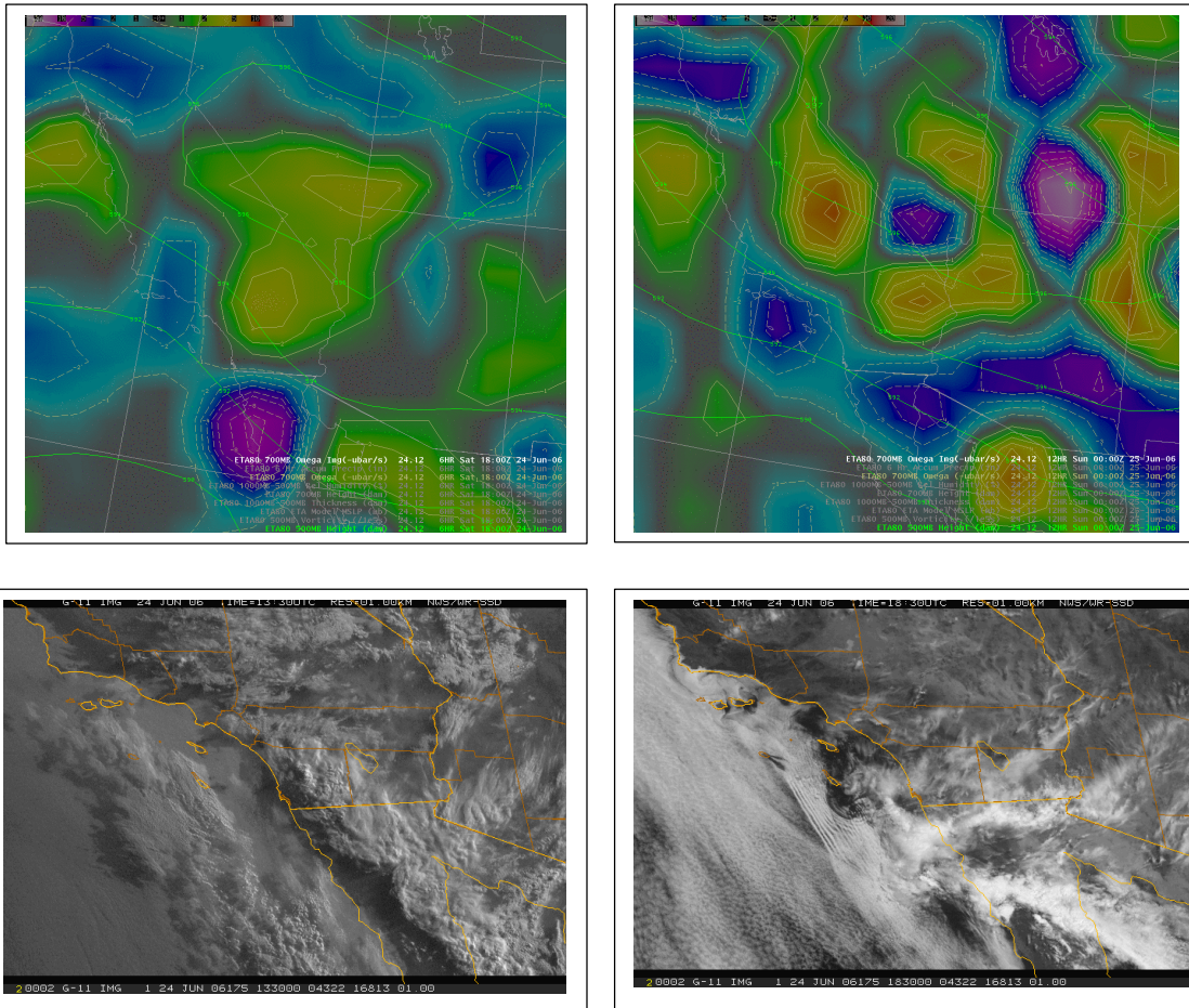
Fig. 8. The subsidence associated with the easterly wave is indicated by the blue to purple region and is moving from east to west across the figures. The upper left is the 06 hour 500 mb heights forecast in decameters (green, solid) and the 700 mb vertical velocity in microbars per second (brown, dashed, and shaded) valid at 1800 UTC 24 June 2006. The upper right is the 12 hour 500 mb heights forecast in decameters (green, solid) and the 700 mb vertical velocity in microbars per second (brown, dashed, and shaded) valid at 0000 UTC 25 June 2006. The lower left is the 1330 UTC 24 June 2006 visible satellite imagery. The lower right is the 1830 UTC 24 June 2006 visible satellite imagery. The peaks in the downward vertical velocity (DVV) over the coastal waters and at the immediate coast during the two time periods were -2.6 and -4.4 respectively. The waves in the low cloud pattern that have been generated by the islands (initially excited by the outflow boundary) appear to be moving westward, even though the clouds moving down the California coast are moving southeastward.
