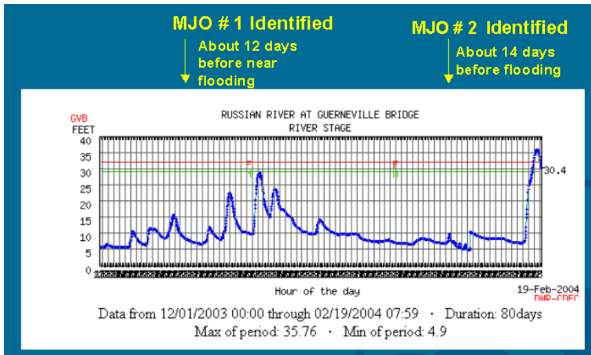
Figure 7. Hydrograph for the Russian river at Guerneville for the period December 1 through February 19, 2004. The red line indicates flood stage.
