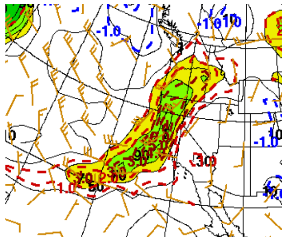
Figure 16: 12Z GFS moisture flux anomalies (red and blue dashed contours).
