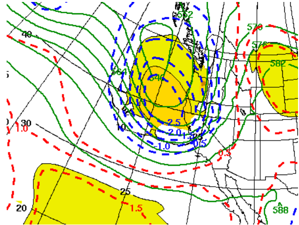
Figure 14: 00Z GFS 500mb heights and standardized anomalies (red and blue dashed contours).
