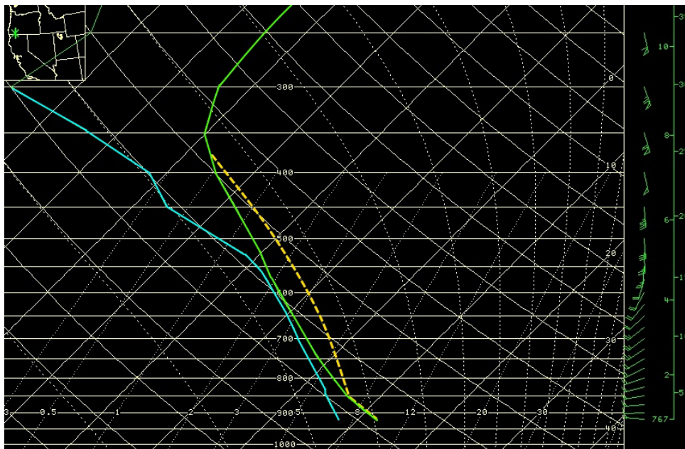
Figure 2: 18Z GFS forecast sounding for 00Z June 5 at Medford. Sounding shows a lifted index of -2.6 and CAPE value of over 500 J/kg.
