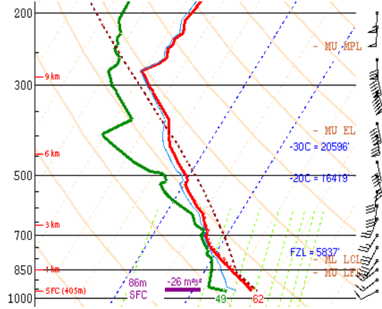
Figure 7: Observed 00Z sounding from KMFR. Observed Cape was over 600 J/kg, 0-3 Km lapse rates were over 8 C/km, but 0-6km shear was 48 kts.
