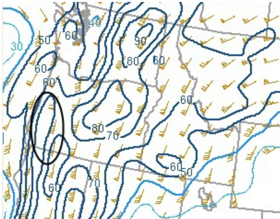
Figure 6: 20Z 0-6km shear from SPC mesoanalysis. Narrow band just inland in southwestern Oregon has values of 70 kts or greater. Note area of local max within oval.
