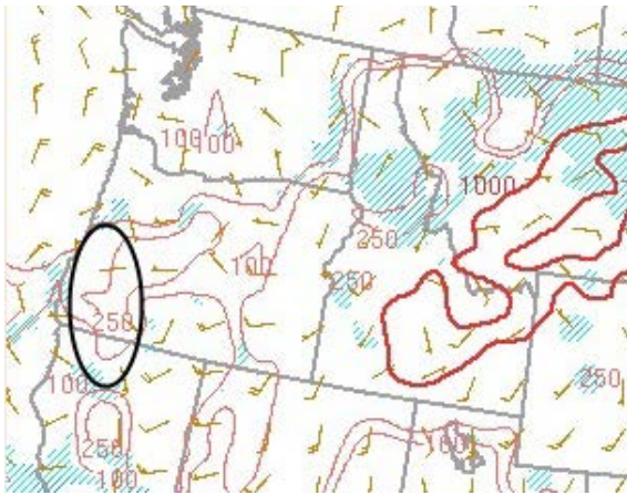
Figure 4: Surface based CAPE from 20Z SPC mesoanalysis. Note area of local max within oval.
