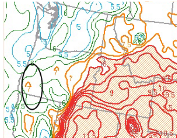
Figure 5: SPC mesoanalysis of 20Z 0-3km lapse rates. Note area of local max within oval.
