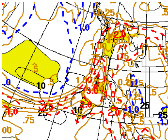
Figure 15: 12Z GFS precipitable water anomalies (red and blue dashed contours).
