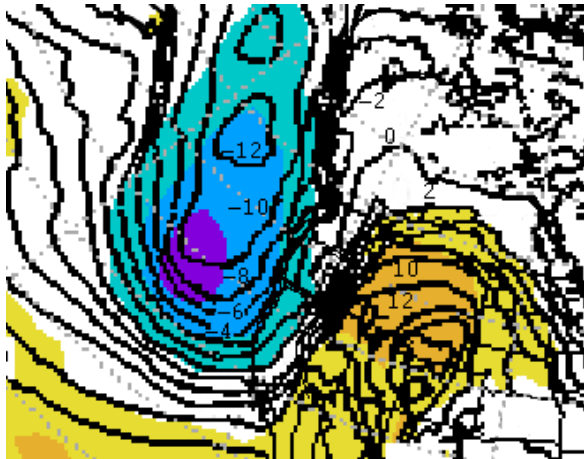
Figure 13: 00Z GFS 700mb temperatures. Standardized anomalies are indicated in color. Note blue and purple shades indicating below normal \sigma . Light blue denotes \sigma of -1, ranging to values of -3 or more within the purple area.
