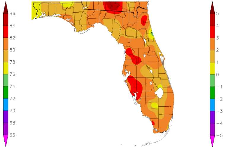
Departure from Normal Temperature (F) 3/1/2024 - 5/31/2024
