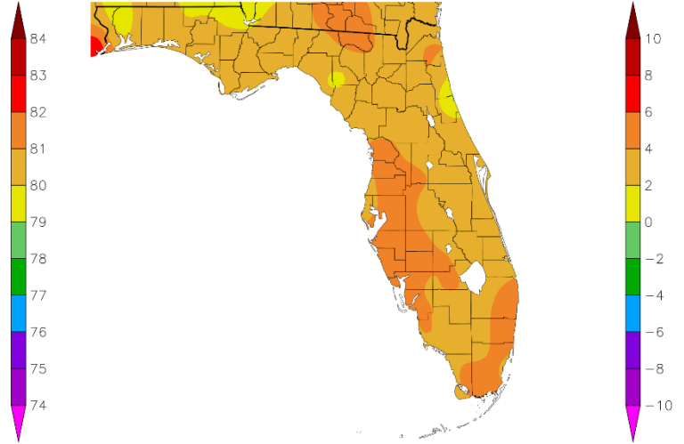
Departure from Normal Temperature (F) 5/1/2024 - 5/31/2024
