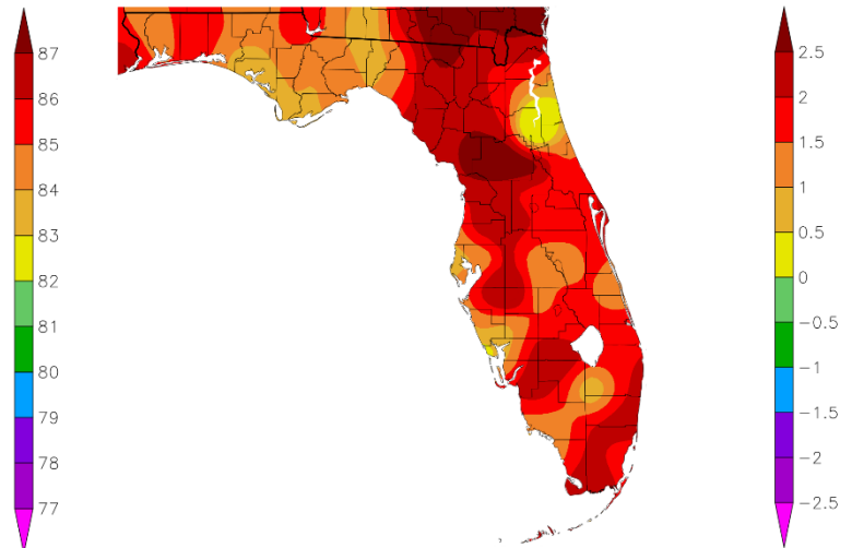
Departure from Normal Temperature (F) 7/1/2026 – 7/31/2026
