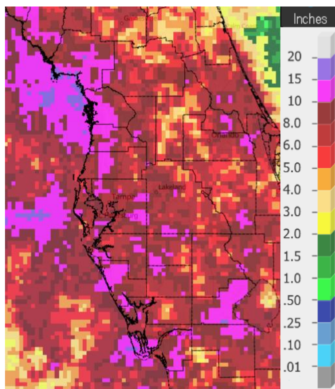
July 2026 Rainfall
