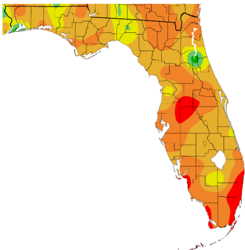
Temperature (F) 7/1/2026 – 7/31/2026
