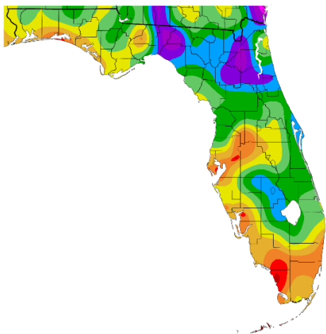
Temperature (F) 8/1/2024 - 8/31/2024
