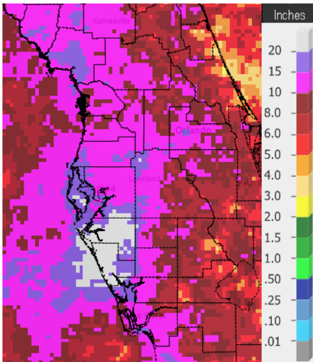
August 2024 Rainfall
