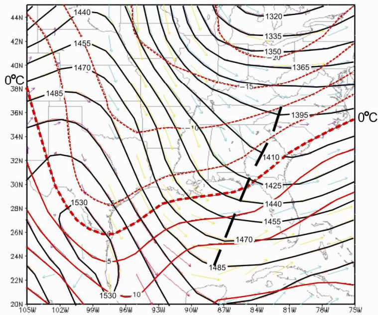
Fig. 10. As in Fig. 3, except for 0000 UTC 13 February 1958.
