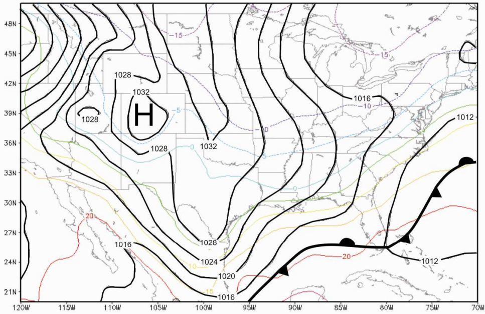
Fig. 5. As in Fig. 2, except for 1200 UTC 12 February 1958.
