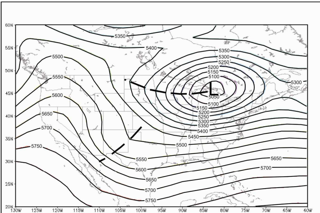
Fig. 1. 500-mb analysis valid for 0000 UTC 12 February 1958. Geopotential heights (every 50 meters) are indicated by black solid lines. Analyzed troughs are shown using standard symbols.
