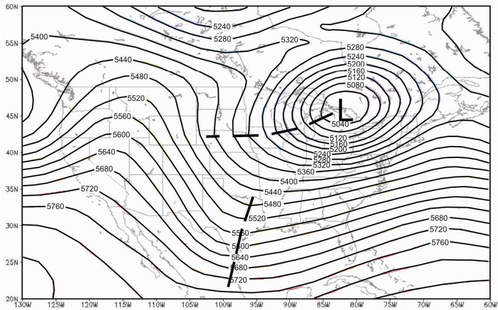
Fig. 4. As in Fig. 1, except for 1200 UTC 12 February 1958.
