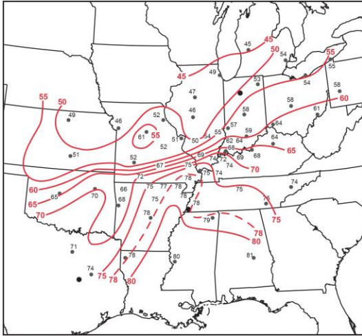
Figure 13: Maximum temperatures (°F) observed on 18 March 1925, contoured at 5°F intervals. Temperature reports from WB forms (small circles are WB stations, larger circles are WB aerological stations), Monthly Climate Summaries by state, and WB cooperative observer reports (plotted at approximate sites). Click image to enlarge.
