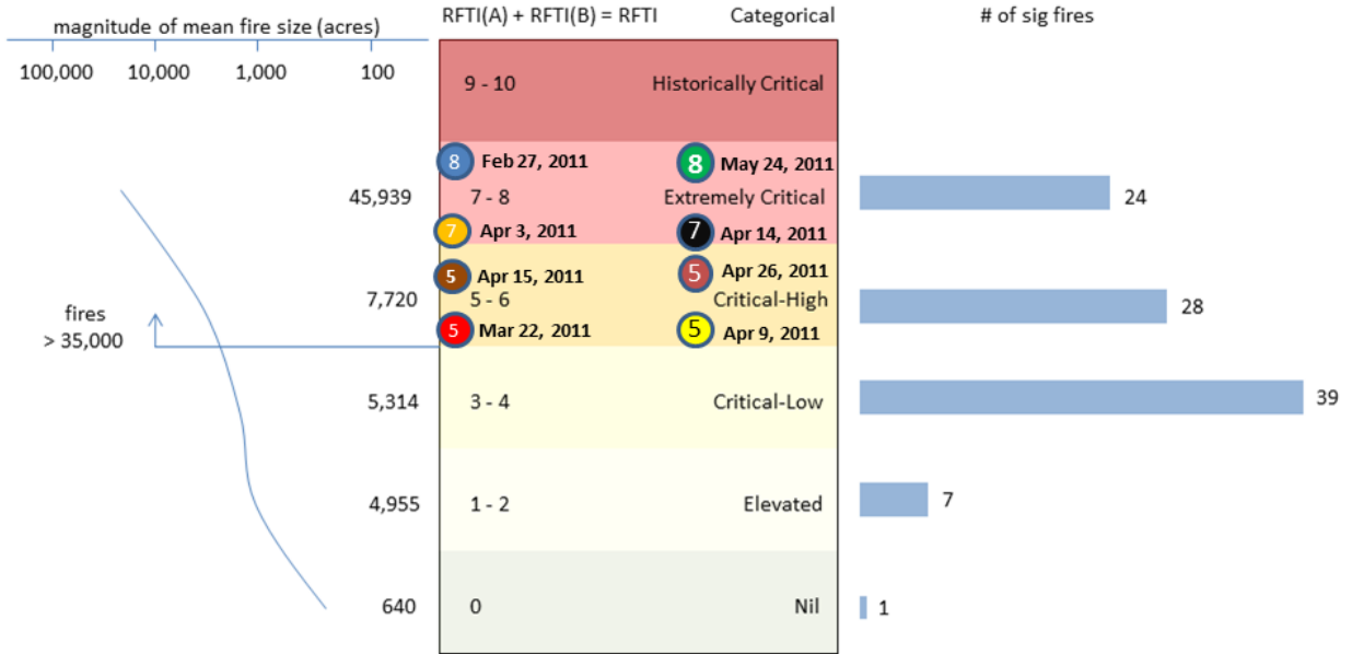
Lubbock (KLBB) RFTI Mod values for the February-May 2011 Southern Plains wildfire outbreaks
