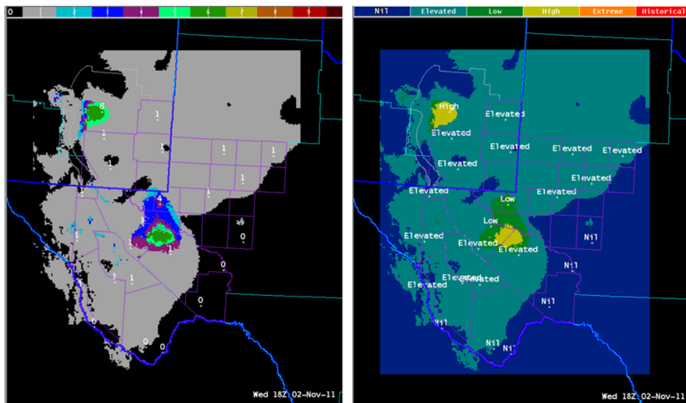
KMAF RFTI Mod forecast grids in GFE for 1800 UTC 2 November 2011
