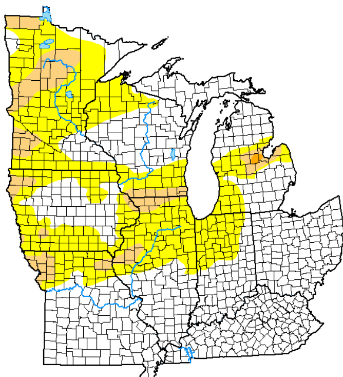
Figure 20. United States Drought Monitor valid 13 May 2025.
