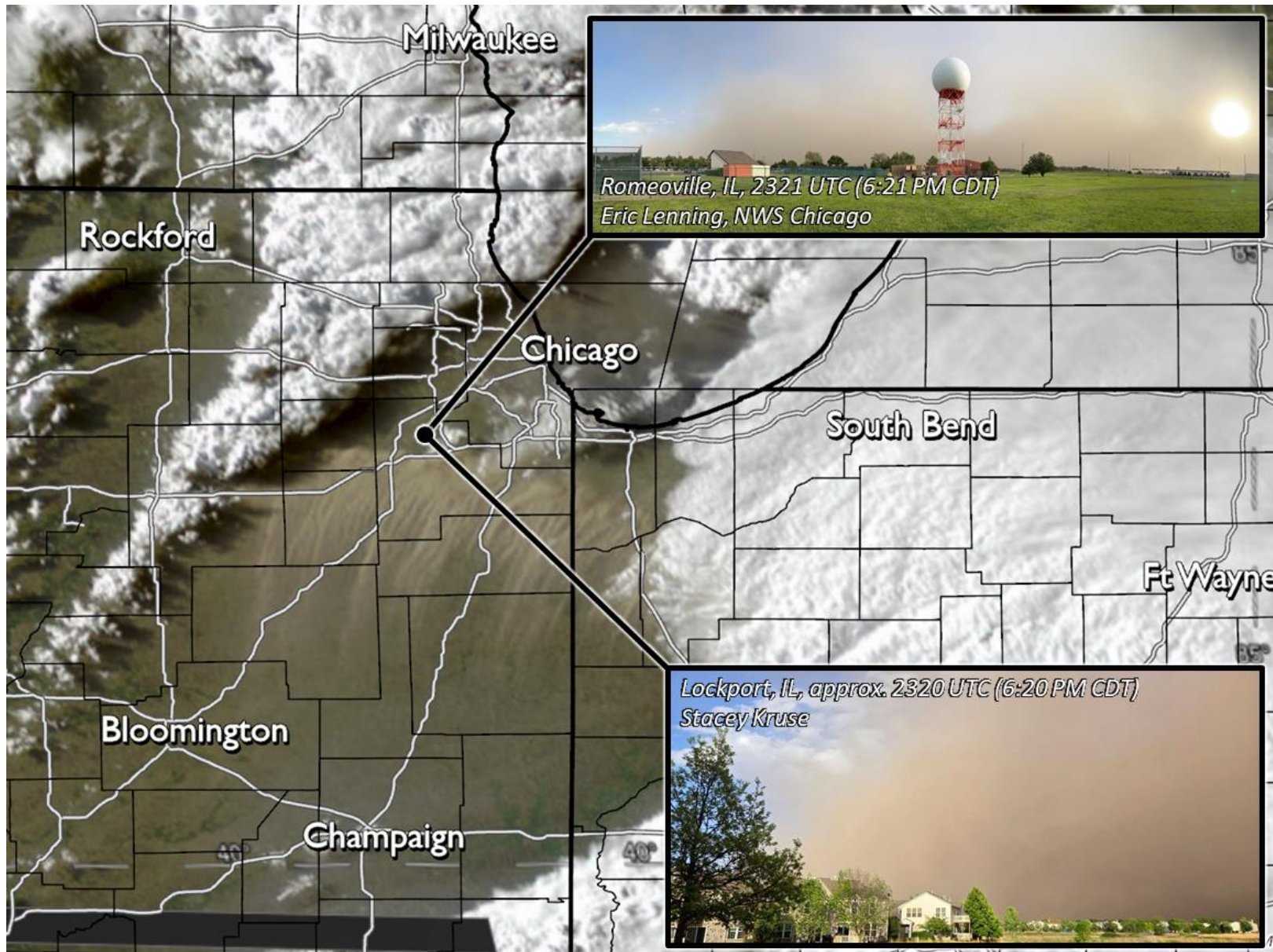
Figure 6. Geo-referenced “true color” satellite image from the GOES-19 satellite valid at 2315 UTC (6:15 PM CDT/7:15 PM EDT) on 16 May 2025. The top right and bottom right insets show the appearance of the dust wall along the leading edge of the dust storm as it neared the NWS Chicago office in Romeoville, Illinois, and Lockport, Illinois, respectively, about 5 minutes later.
