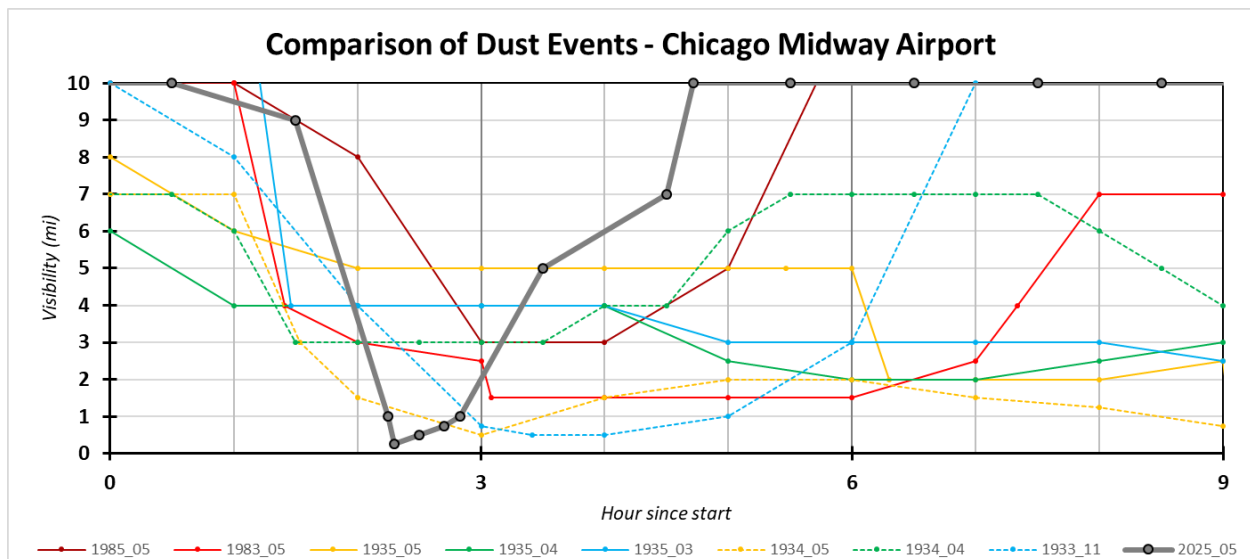
Figure 21. Visibility observations for the known blowing dust and dust storm events impacting Chicago. Visibility observations are from Chicago Midway Airport (MDW).
