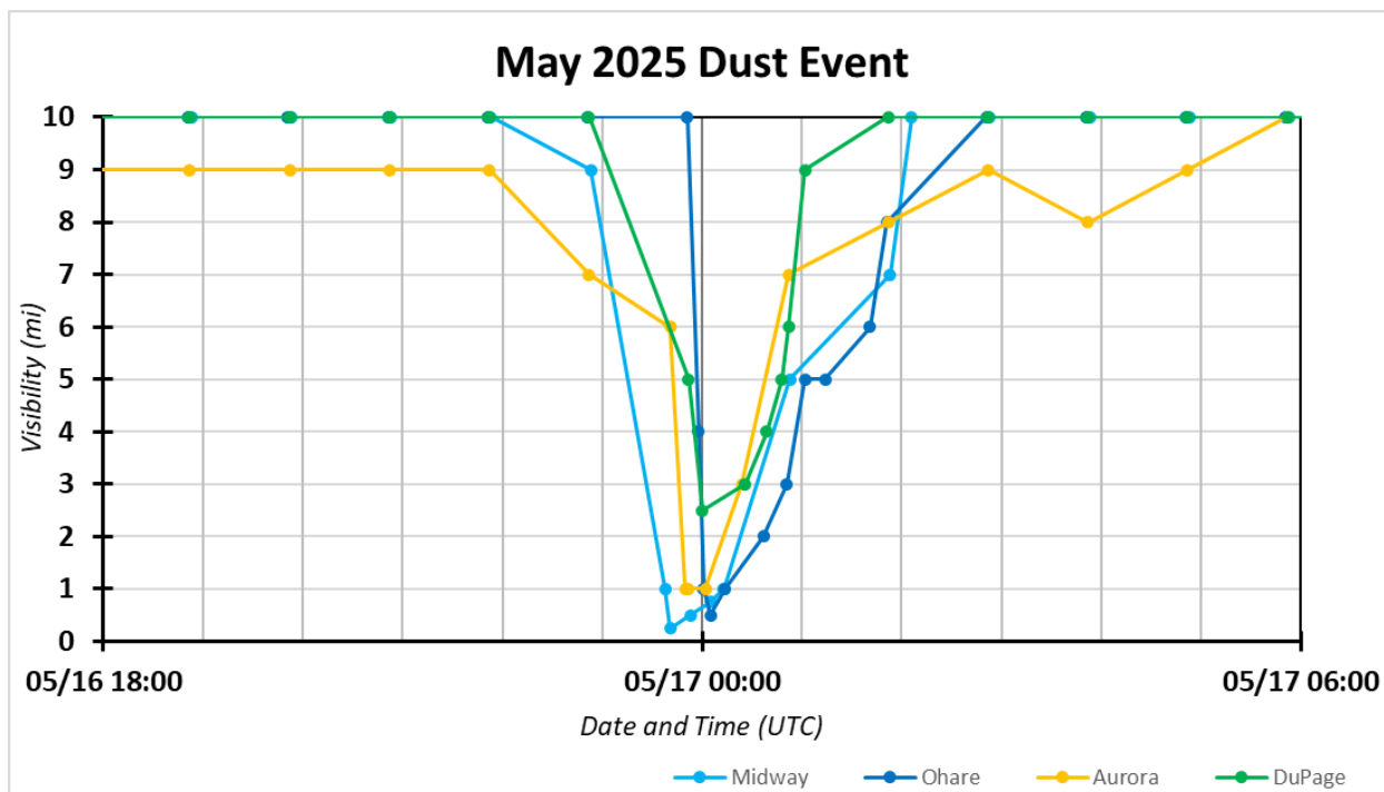
Figure 13. Visibility observations around the Chicago Metropolitan Area collected during the 16 May 2025 dust storm event.
