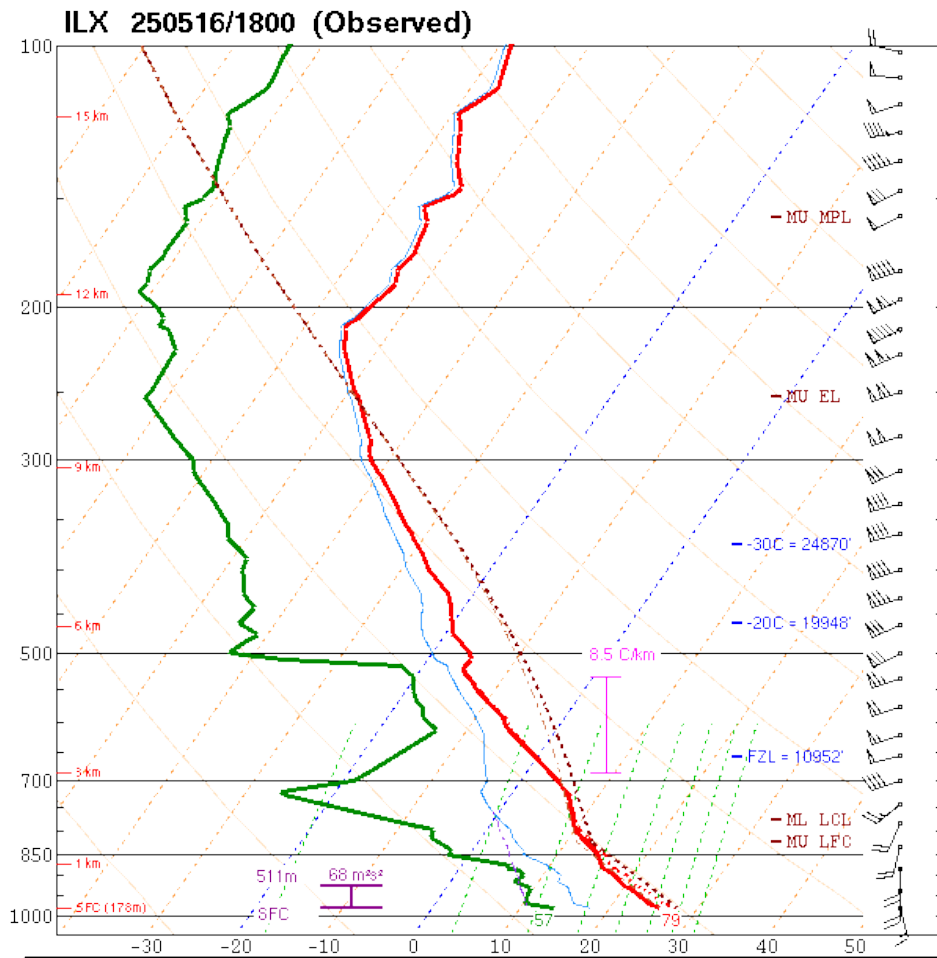
Figure 14. Sounding from Lincoln, Illinois (ILX), from 1800 UTC (1:00 PM CDT) on 16 May 2025. From SPC soundings page ( https://www.spc.noaa.gov/exper/soundings/ ).
