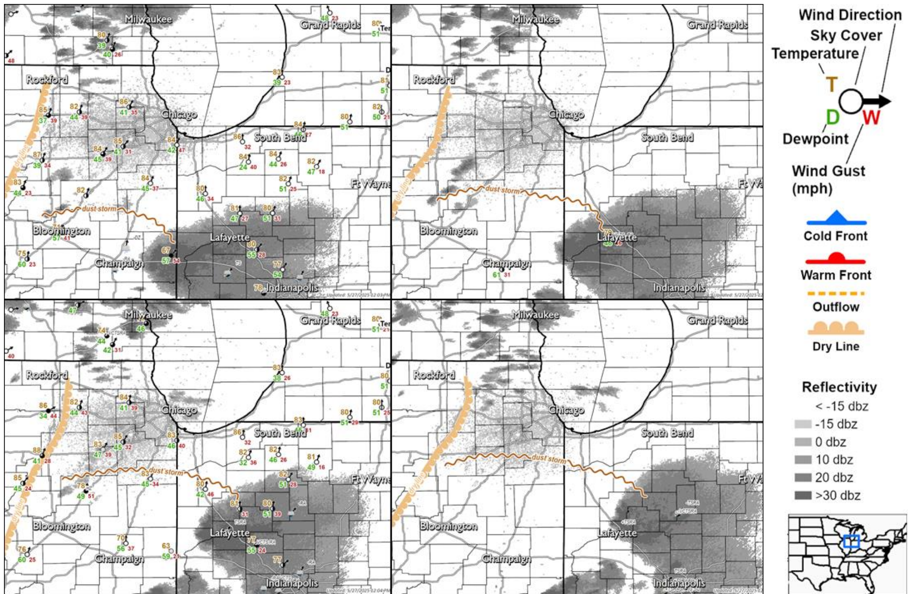
Figure 9. Surface weather features and dust storm progression analyzed at 15-minute intervals beginning at 2215 UTC (5:15 PM CDT/6:15 PM EDT) on 16 May 2025. Maps are in left to right, top to bottom order. Radar imagery in grayscale added as an underlay.
