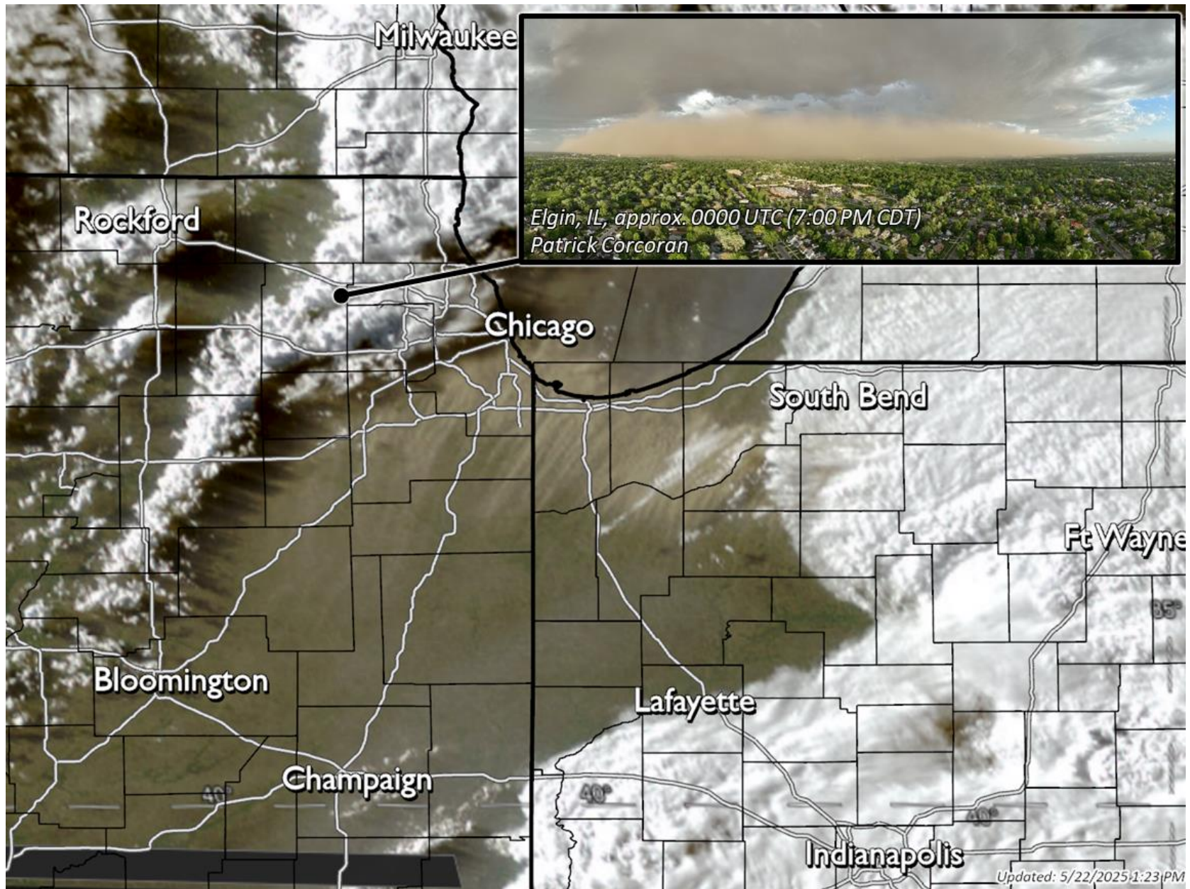
Figure 7. Geo-referenced "true color" satellite image from the GOES-19 satellite valid at 2346 UTC (6:46 PM CDT/7:46 PM EDT) on 16 May 2025. The inset shows the appearance of the dust wall along the leading edge of the dust storm as it neared Elgin, Illinois, approximately 15 minutes later.
