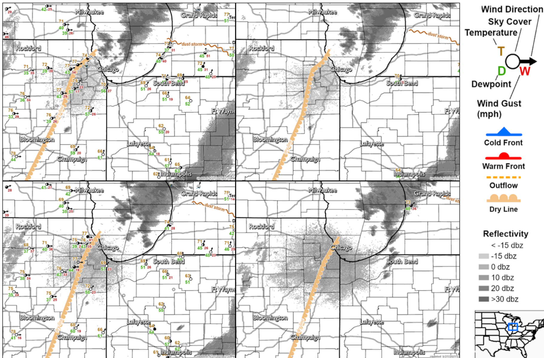
Figure 12. Surface weather features and dust storm progression analyzed at 15-minute intervals beginning at 0115 UTC on 17 May 2025 (8:15 PM CDT/9:15 PM EDT on 16 May). Maps are in left to right, top to bottom order. Radar imagery in grayscale added as an underlayer.
