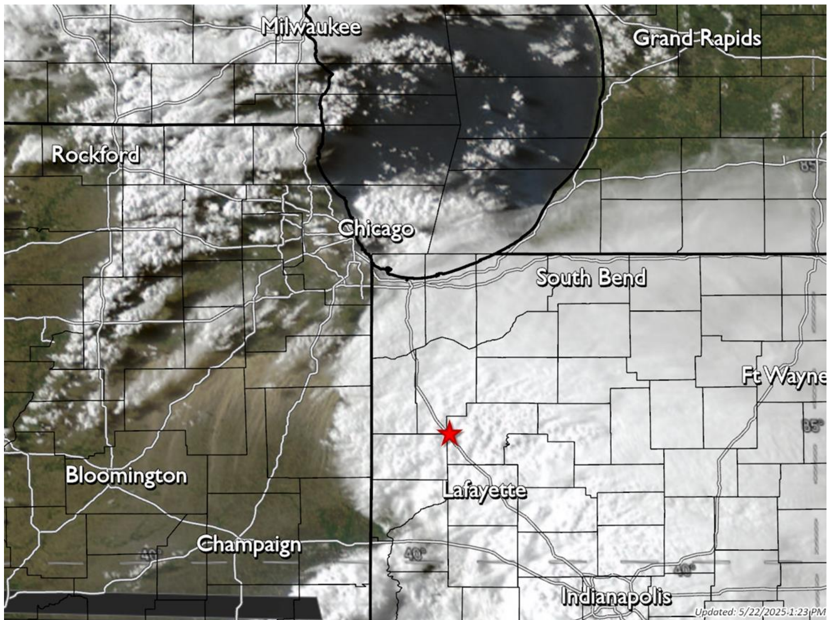
Figure 4. Geo-referenced “true color” satellite image from the GOES-19 satellite valid at 2246 UTC (5:46 PM CDT/6:46 PM EDT) on 16 May 2025. The red star indicates the location of the photos in Figure 5, taken at approximately the same time.
