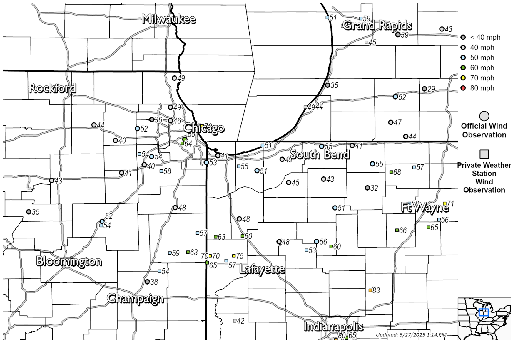
Figure 18. Peak observed wind gusts, in mph, from the dust storm that occurred on 16 May 2025. Observations from private weather stations, marked with small squares, come from equipment of widely-varying type, quality, and siting, and should be used with caution.
