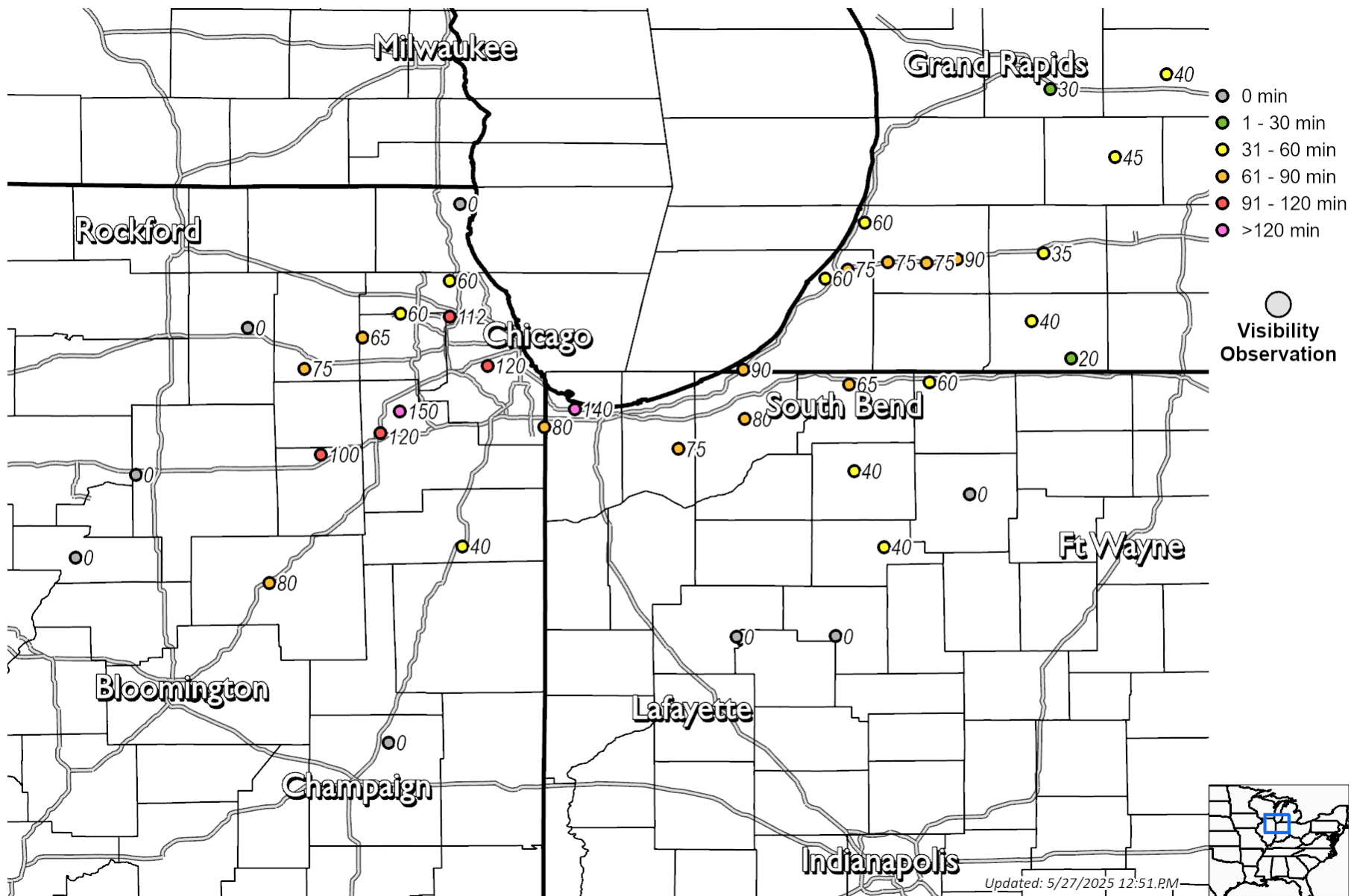
Figure 16. Duration (in minutes) of reduced visibilities from the dust storm that occurred on 16 May 2025.
