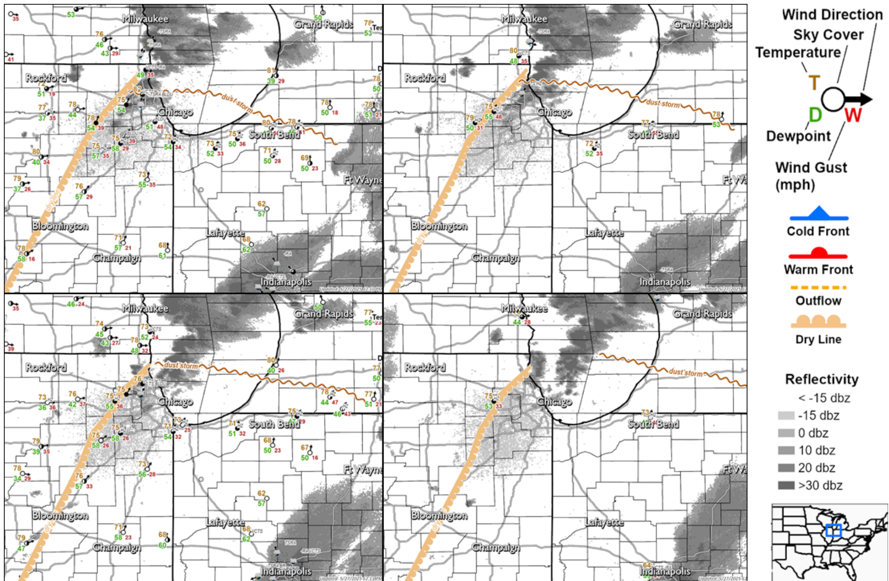
Figure 11. Surface weather features and dust storm progression analyzed at 15-minute intervals beginning at 0015 UTC on 17 May 2025 (7:15 PM CDT/8:15 PM EDT on 16 May). Maps are in left to right, top to bottom order. Radar imagery in grayscale added as an underlayer.
