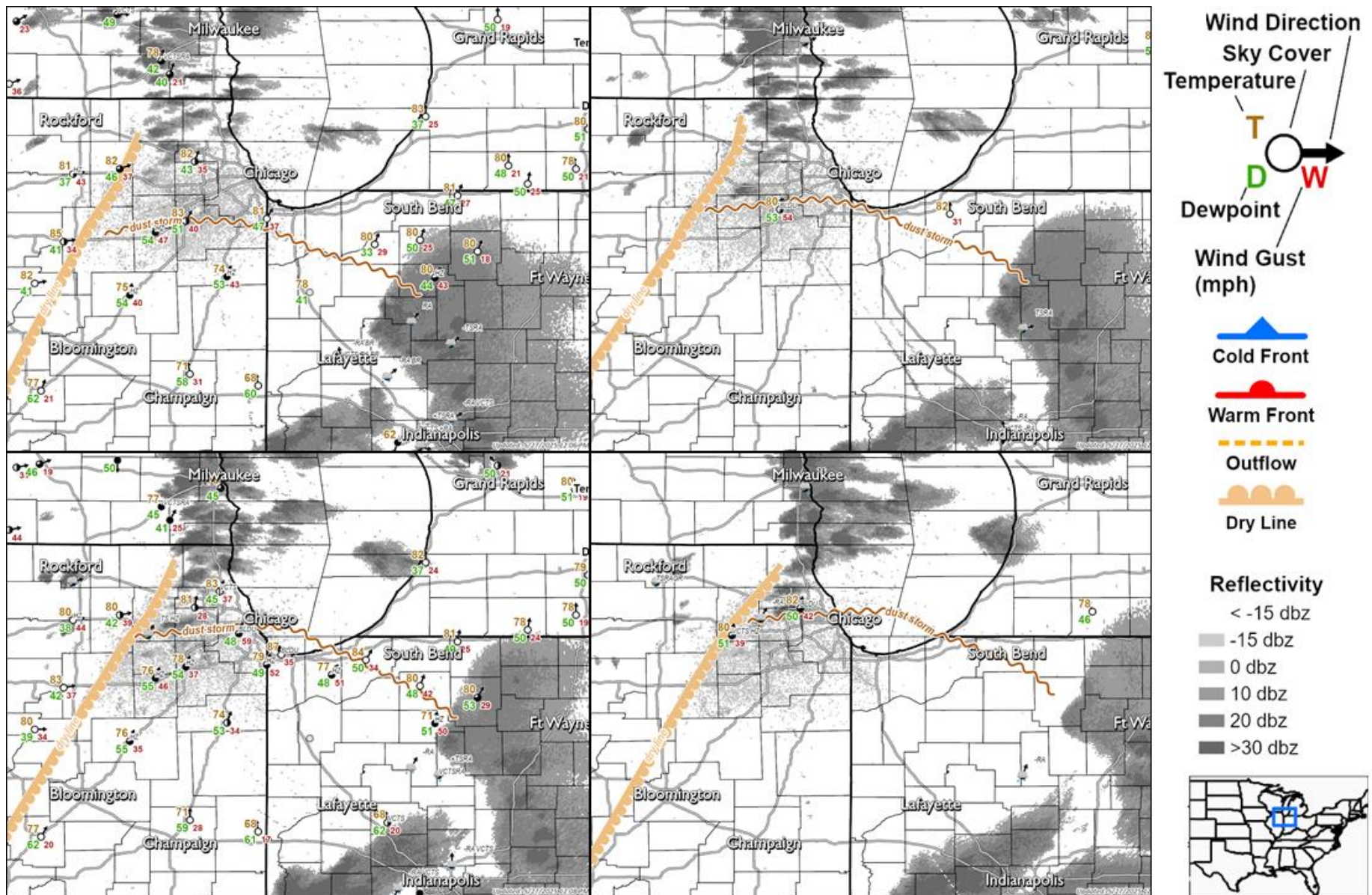
Figure 10. Surface weather features and dust storm progression analyzed at 15-minute intervals beginning at 2315 UTC (6:15 PM CDT/7:15 PM EDT) on 16 May 2025. Maps are in left to right, top to bottom order. Radar imagery in grayscale added as an underlay.
