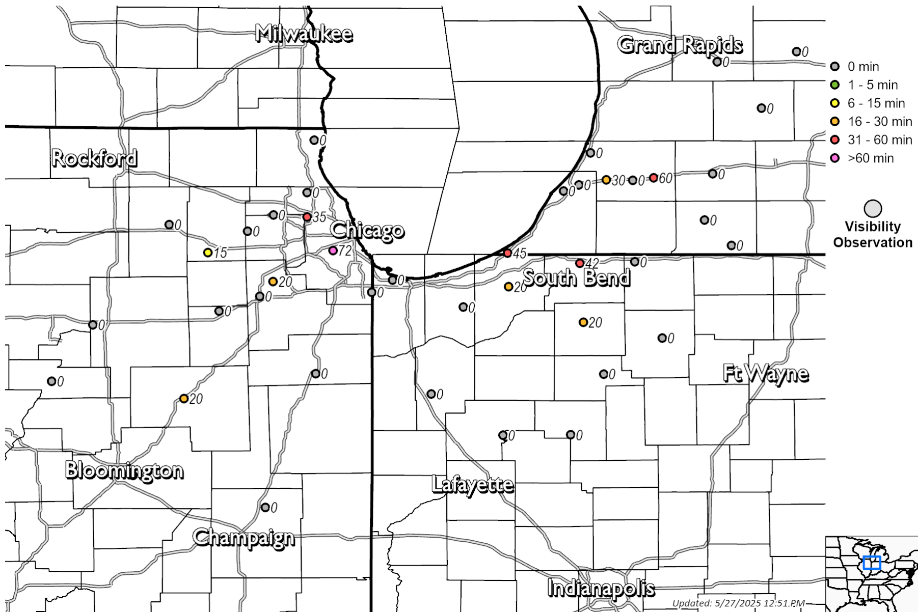
Figure 17. Duration, in minutes, of significantly reduced visibilities (<1 mile) from the dust storm that occurred on 16 May 2025.
