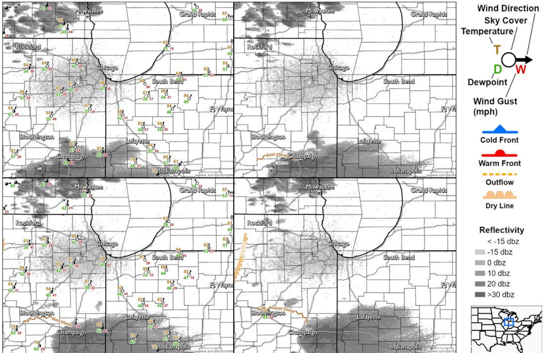
Figure 8. Surface weather features and dust storm progression analyzed at 15-minute intervals beginning at 2115 UTC (4:15 PM CDT/5:15 PM CDT) on 16 May 2025. Maps are in left to right, top to bottom order. Radar imagery in grayscale added as an underlay.
