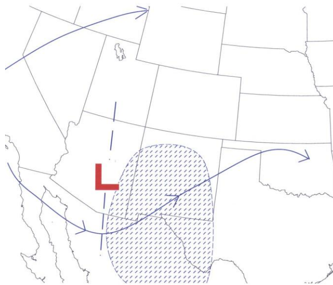
Fig.11. Middle- and upper-tropospheric features associated with Type IV El Paso CWA flash floods. Details the same as Fig. 5.
