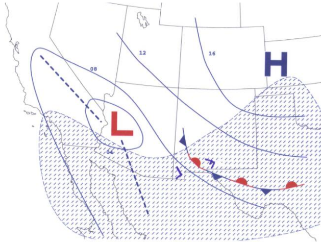
Fig.4. Surface pattern for a typical El Paso CWA Type I flash flood. Surface low and high pressure centers indicated by L and H respectively. Dashed line shows position of surface trough axis. Conventional frontal symbols used. Solid lines represent isobars with pressure given in millibars ( minus 1000). Dewpoints exceed 55 °F in the hatched areas.
