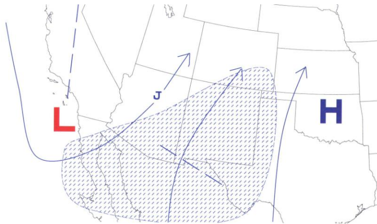
Fig. 7. Middle- and upper-tropospheric features associated with Type II El Paso CWA flash floods. L and H indicate 500-mb minimum and maximum geopotential height centers respectively. Other details the same as Fig. 5.
