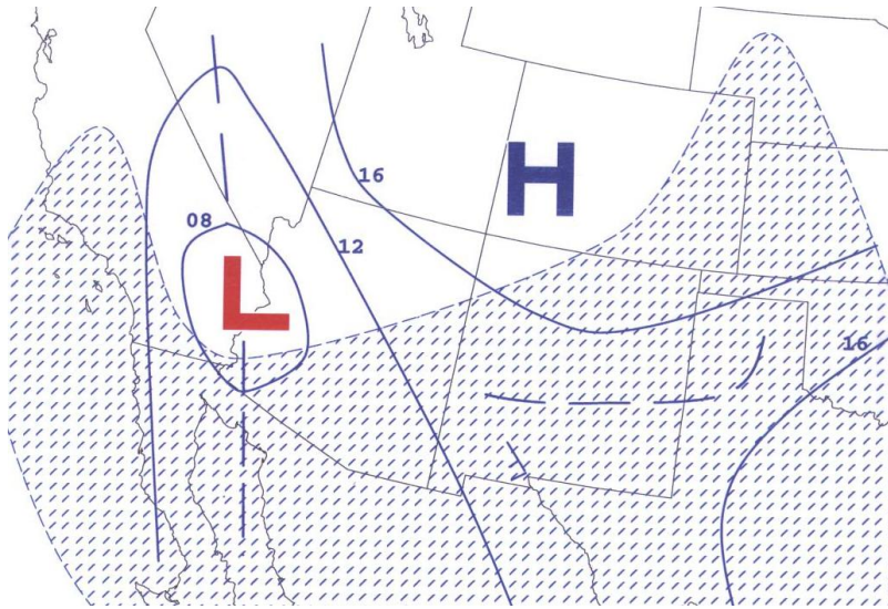
Fig. 8. Surface pattern for Type III flash floods. Details same as Fig. 4.
