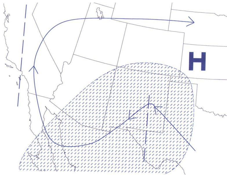
Fig. 9. Middle- and upper-tropospheric features associated with Type III El Paso CWA flash floods. Details the same as Fig. 5.
