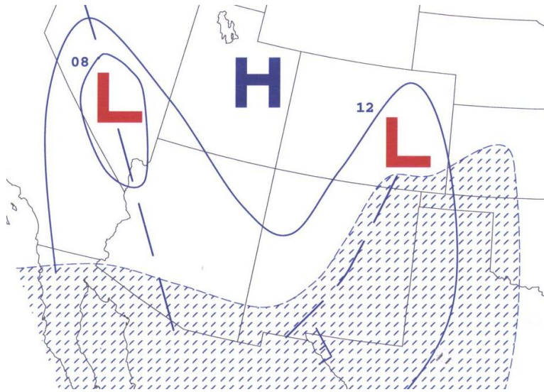
Fig. 10. Surface pattern for Type IV flash floods. Details same as Fig. 4.
