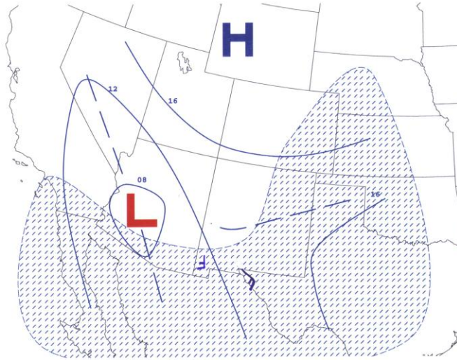
Fig. 6. Surface pattern for a typical El Paso CWA Type II flash floods. Details are the same as in Fig. 4.
