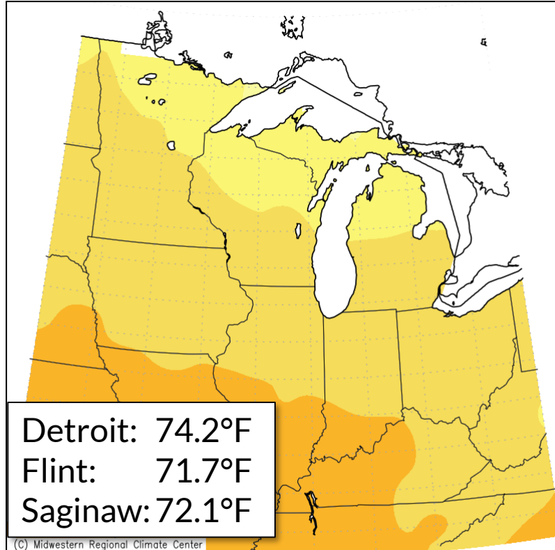
Average Temperature (°F) June 1, 2021 to August 31, 2021
