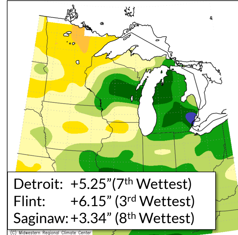
Accumulated Precipitation: Percent of Mean June 1, 2021 to August 31, 2021
