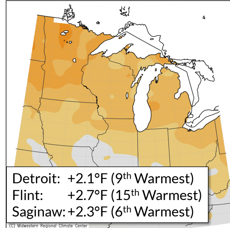
Average Temperature (°F): Departure from Mean June 1, 2021 to August 31, 2021
