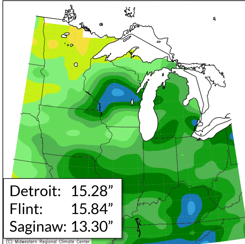
Accumulated Precipitation (in) June 1, 2021 to August 31, 2021
