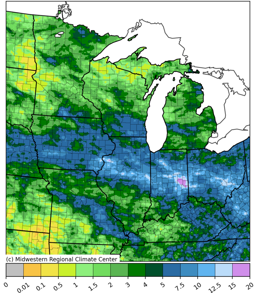
Accumulated Precipitation (in) August 01, 2026 to August 31, 2026
