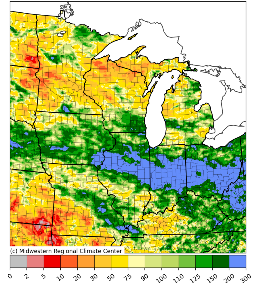
Accumulated Precipitation: Percent of 1991-2020 Normals August 01, 2026 to August 31, 2026
