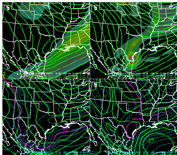
Figure 4. As in Fig. 3, except for 1200 UTC.
