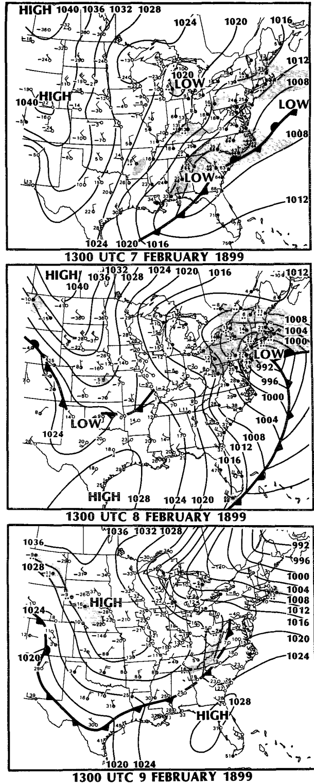
FIG. 1. Sea level pressure (hPa) and surface frontal analyses at (a) 1300 UTC 7 February 1899, (b) 1300 UTC 8 February 1899, and (c) 1300 UTC 9 February 1899. Station plots depict cloud cover, temperature (°F), precipitation type and intensity, and wind velocity. Precipitation areas are shaded. Isobars were analyzed using observed sea level pressures (not plotted).
