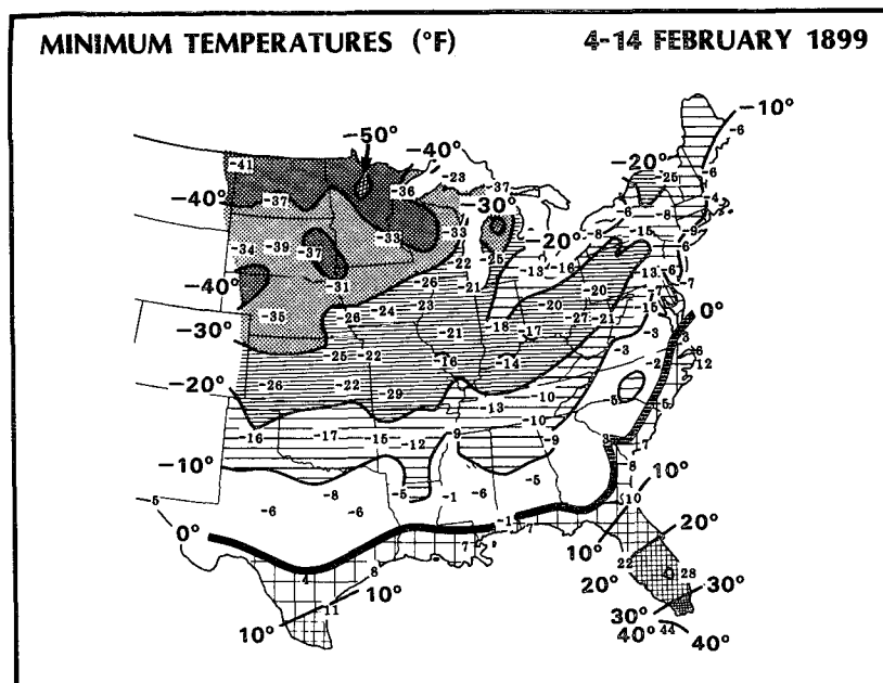
FIG. 7. Minimum temperatures ( ^{\circ}\text{F} ) observed during the period 4–14 February 1899 over the central, eastern, and southern United States. Analyses were generated from measurements at main Weather Bureau stations and from reports of voluntary and cooperative observers. Isotherms are drawn at 10^{\circ}\text{F} ( 5.6^{\circ}\text{C} ) intervals and reflect reports from approximately 1500 cooperative observers. Temperatures at the main Weather Bureau stations are plotted.
