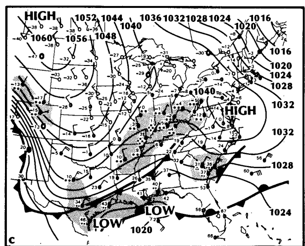
FIG. 2. Sea level pressure (hPa) and surface frontal analyses at (a) 1300 UTC 10 February 1899, (b) 0100 UTC 11 February 1899, and (c) 1300 UTC 11 February 1899. See Fig. 1 caption for details.
