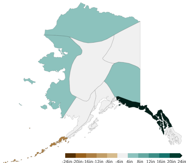
Right: Alaska Divisional Precipitation Anomaly from October 2023-September 2024 Period: 1925-2024
