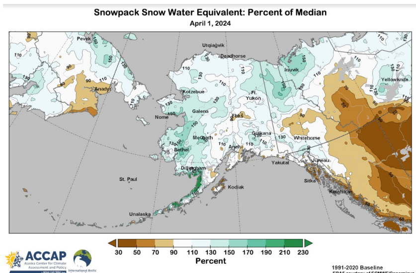
Snow Water Equivalent percent of normal for April 1st 2024 from the ERA5 Reanalysis 1991-2020. Courtesy of the Alaska Center for Climate Assessment and Policy ( https://uaf-accap.org )
