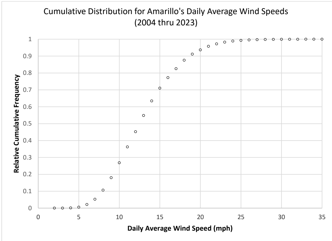
Figure 1. The cumulative distribution of Amarillo's daily average wind speeds
