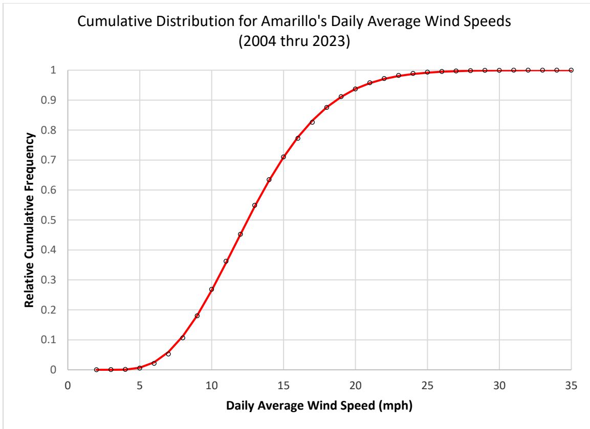
Figure 2. The cumulative distribution with the best fit Weibull Curve
